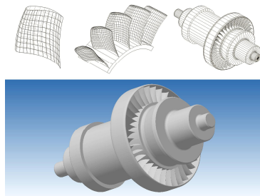
3D Assemblies in MEDUSA4
