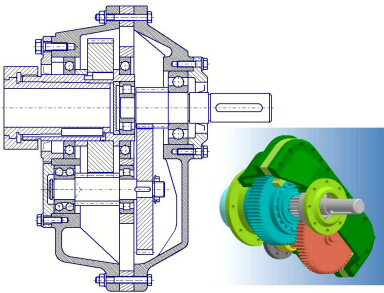
Drawing of an assembly with corresponding 3D view
